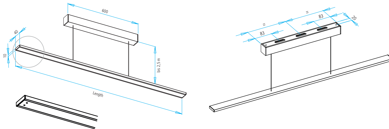
Version with sensor switch
